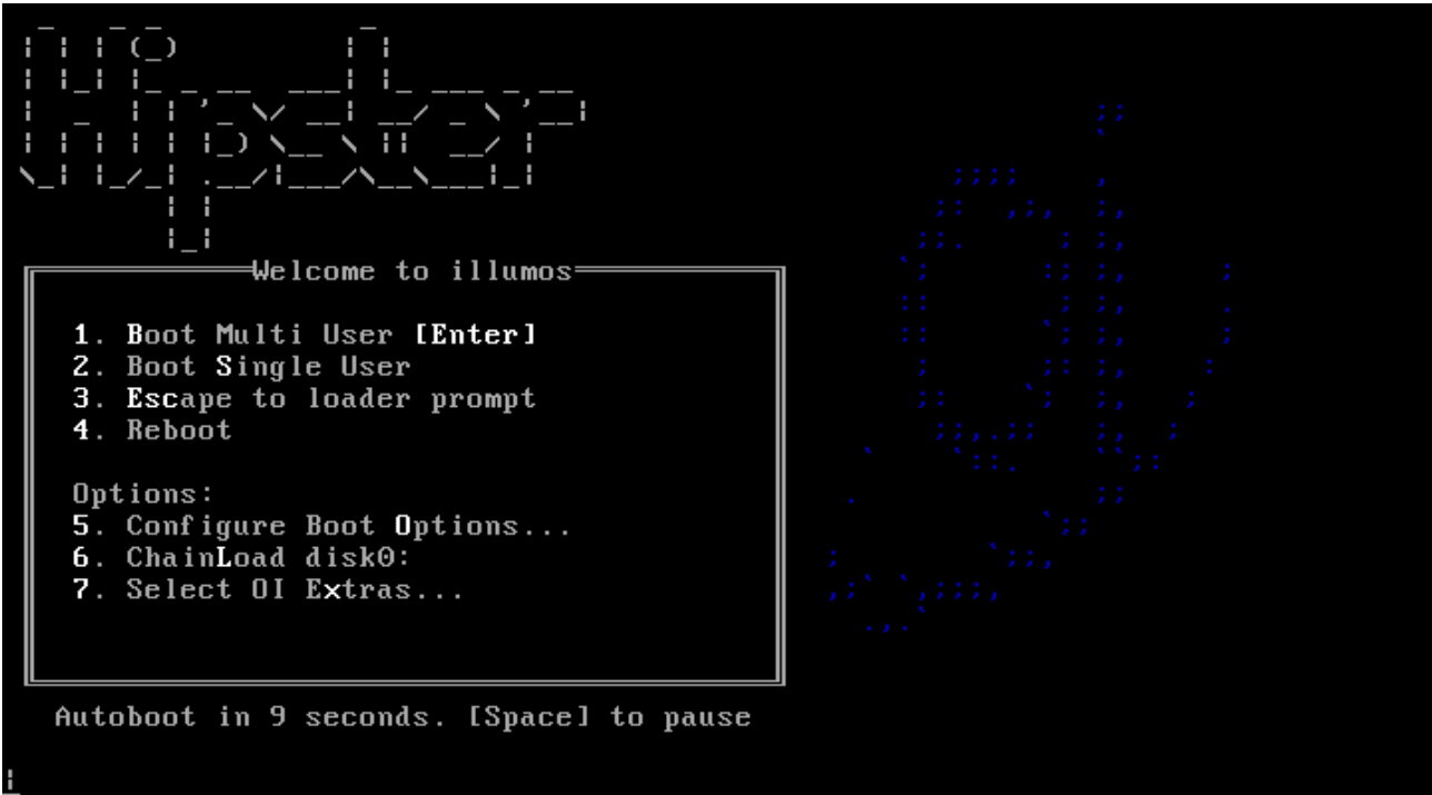
Figure 1: forth_menu
