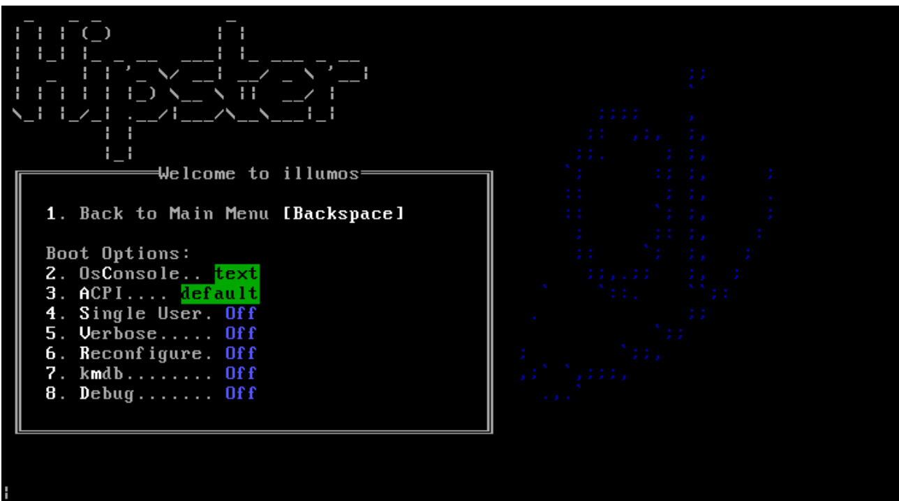
Figure 2: forth_boot_menu_options
