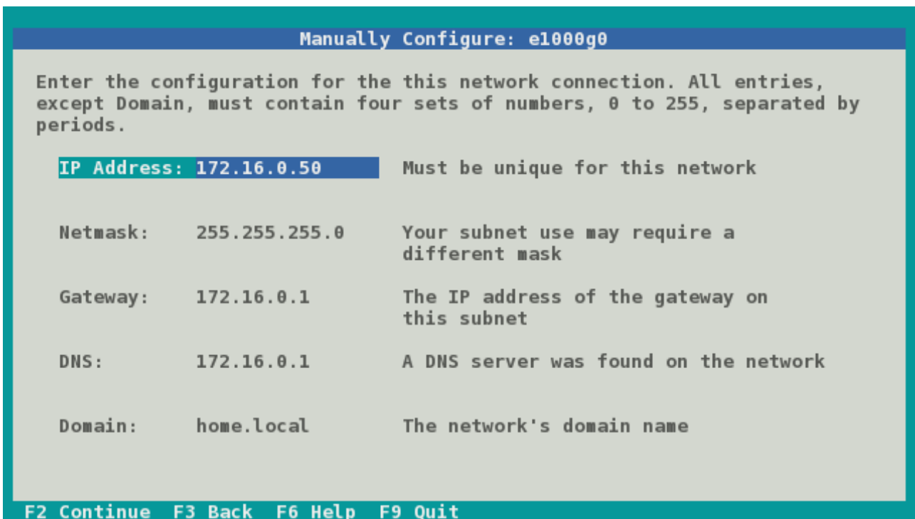
Figure 23: Network 3
