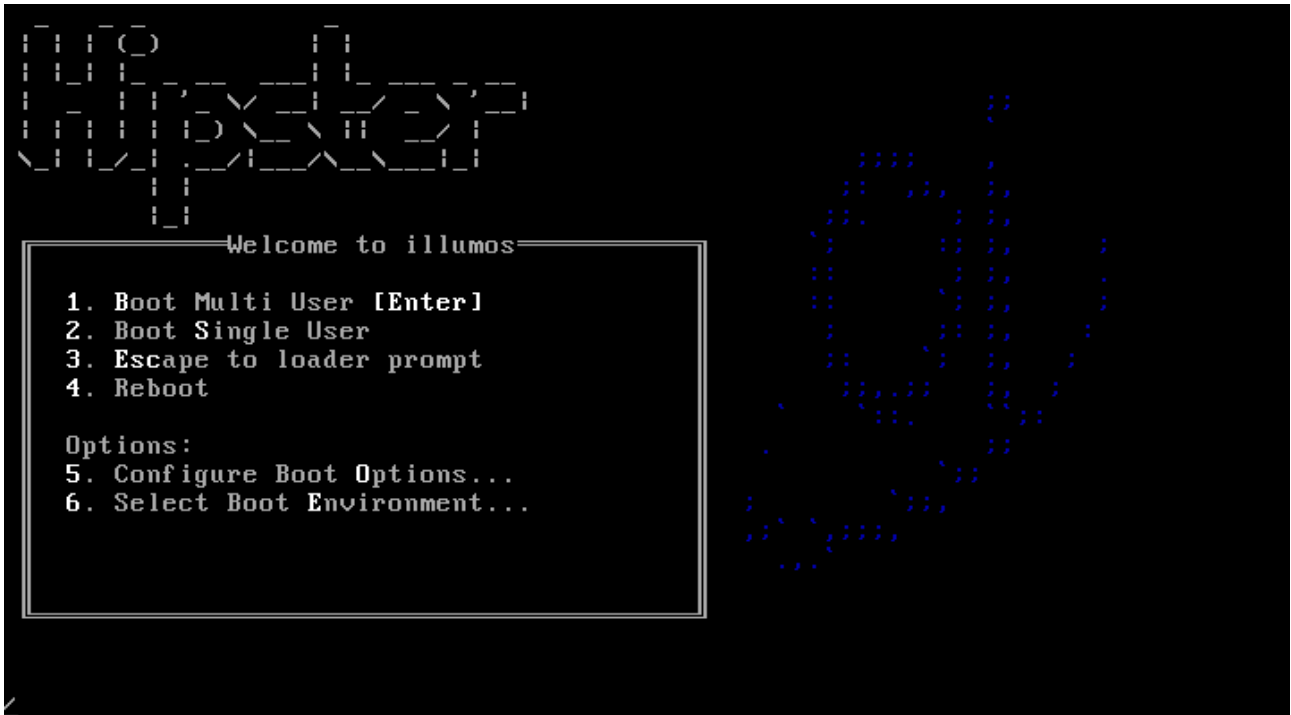
Figure 34: forth_menu
