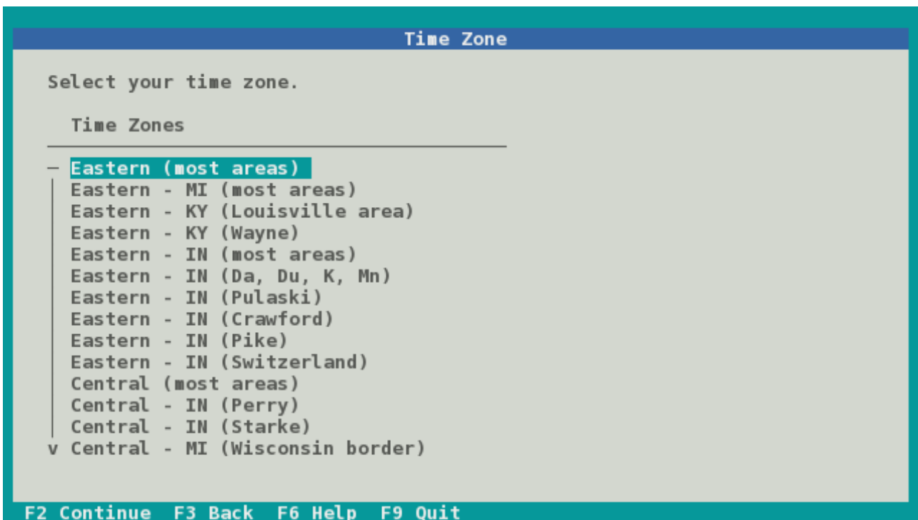
Figure 26: Time Zone
