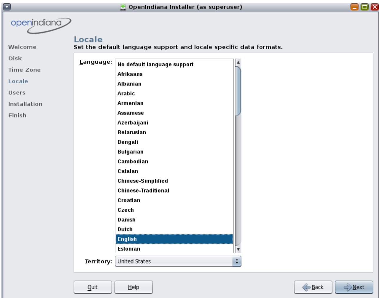
Figure 10: Locale
