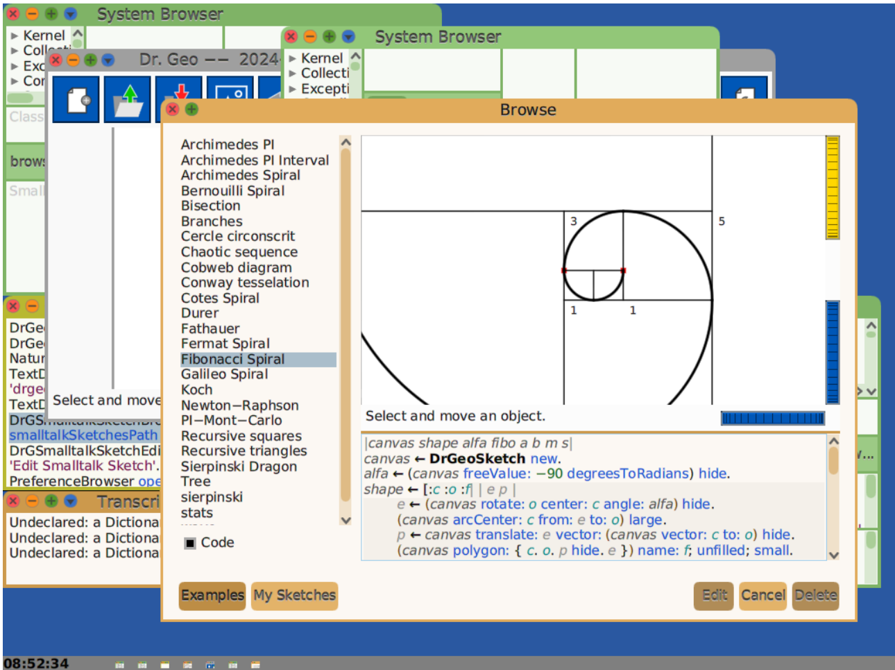
Figure 6: cuis drgeo
