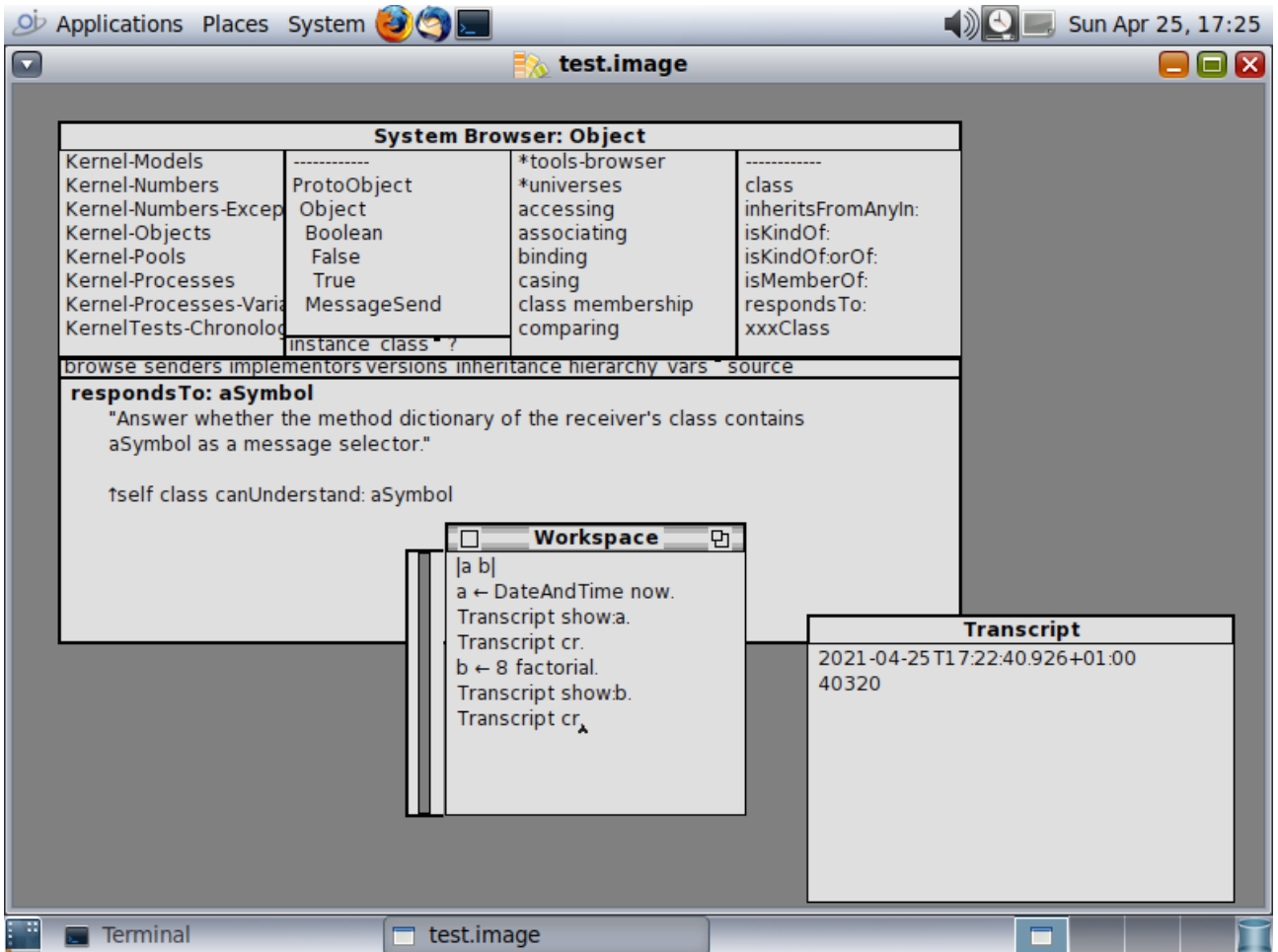
Figure 1: mvc
