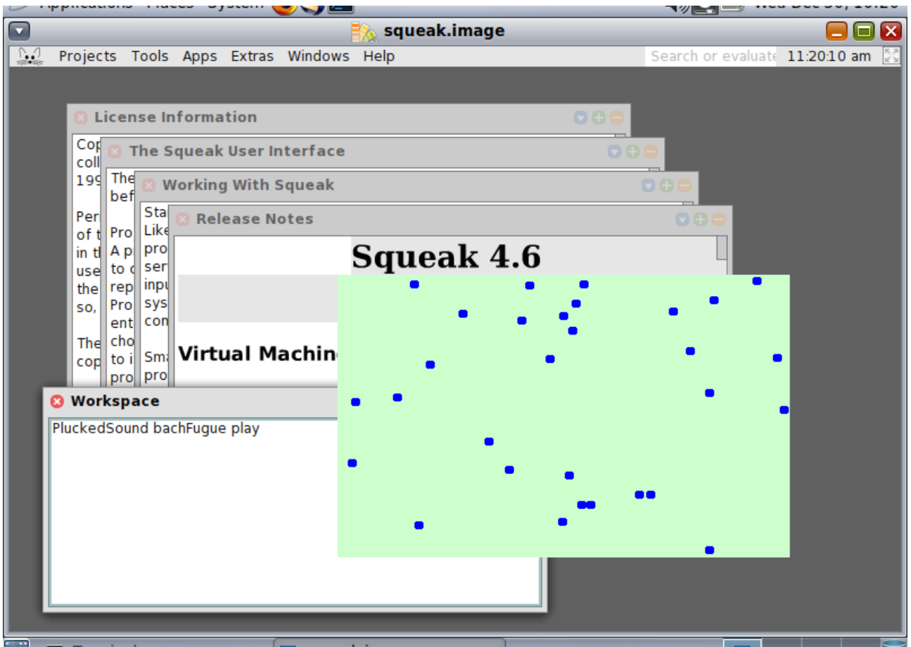
Figure 2: bouncing atoms
